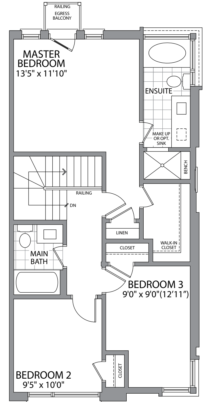
THIRD FLOOR ELEVATION A & B
