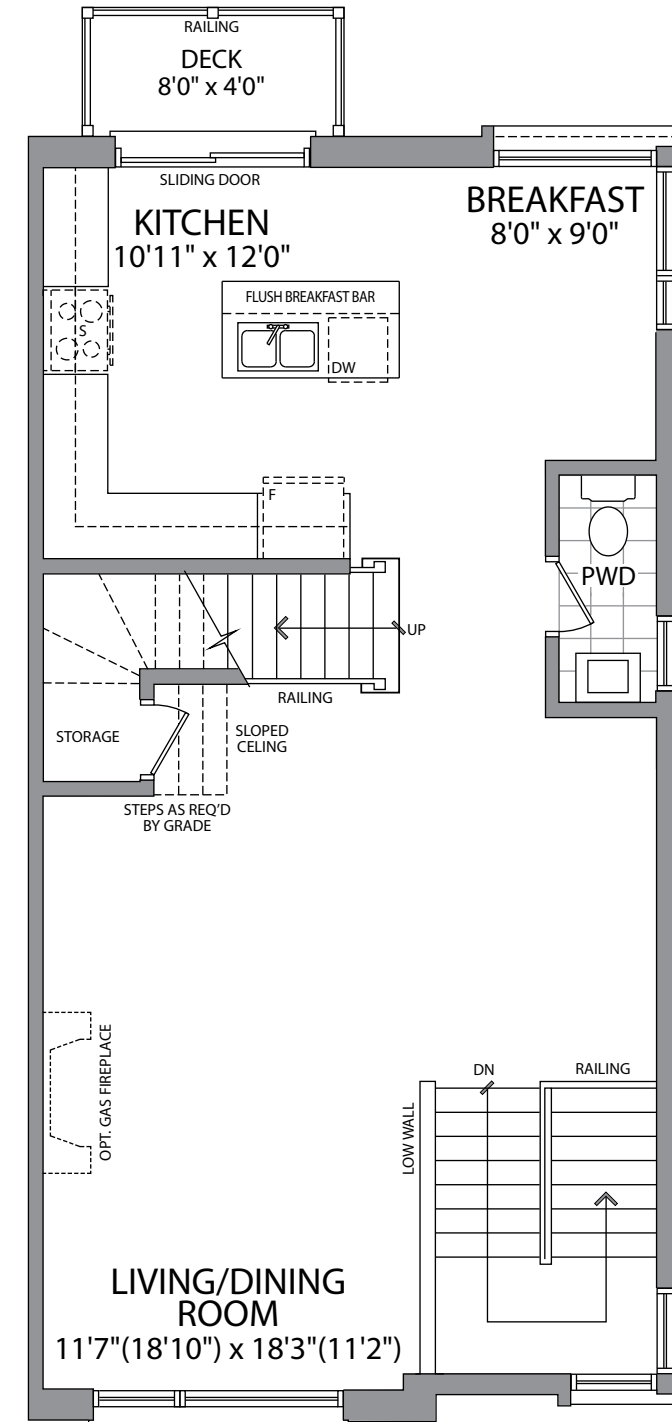
SECOND FLOOR ELEVATION A & B
