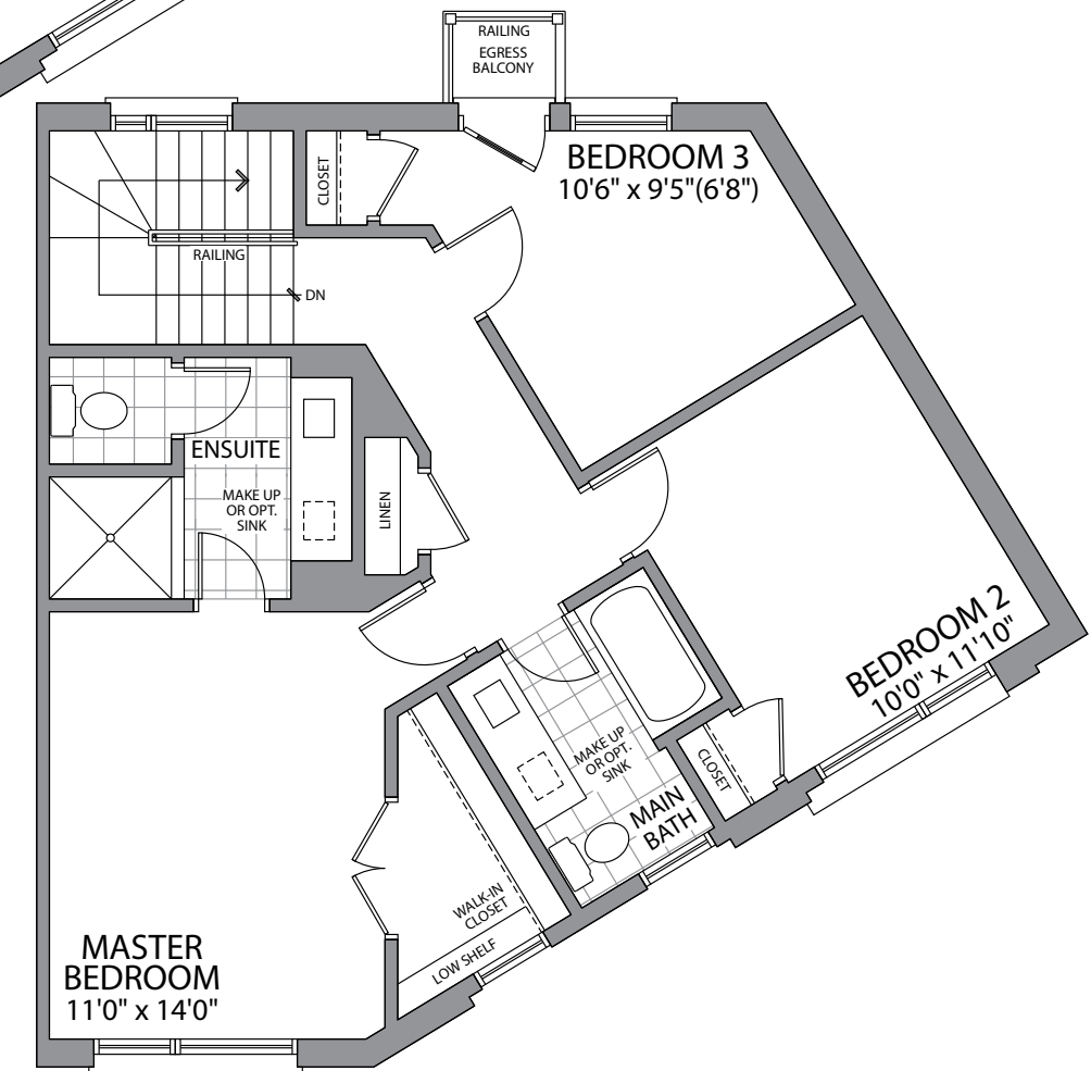
THIRD FLOOR ELEVATION A & B
