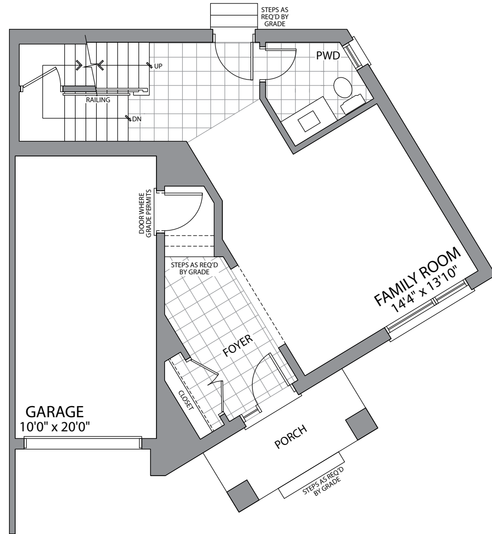
FIRST FLOOR ELEVATION A & B
