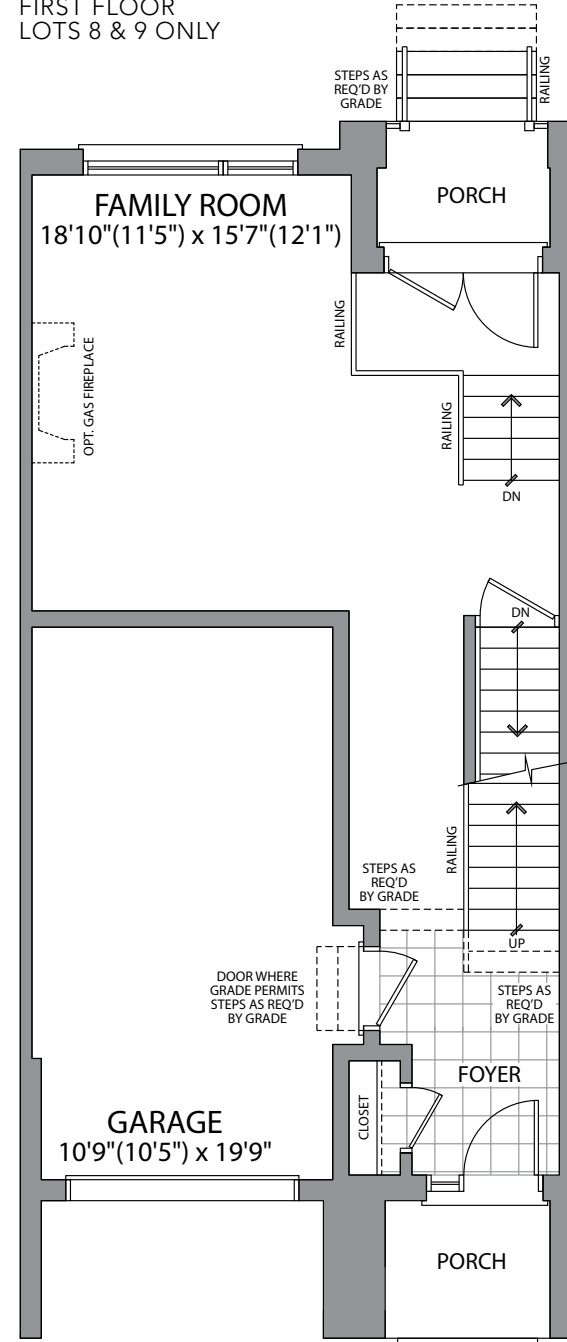
FIRST FLOOR ELEVATION A & B
