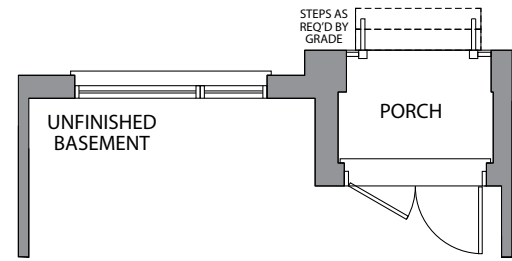
BASEMENT LOTS 8 & 9 ONLY
