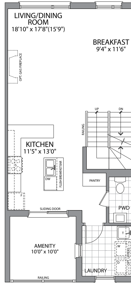
SECOND FLOOR ELEVATION A & B
