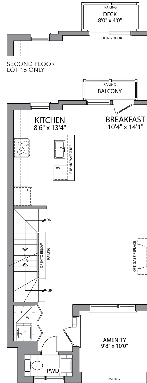
SECOND FLOOR ELEVATION A & B
