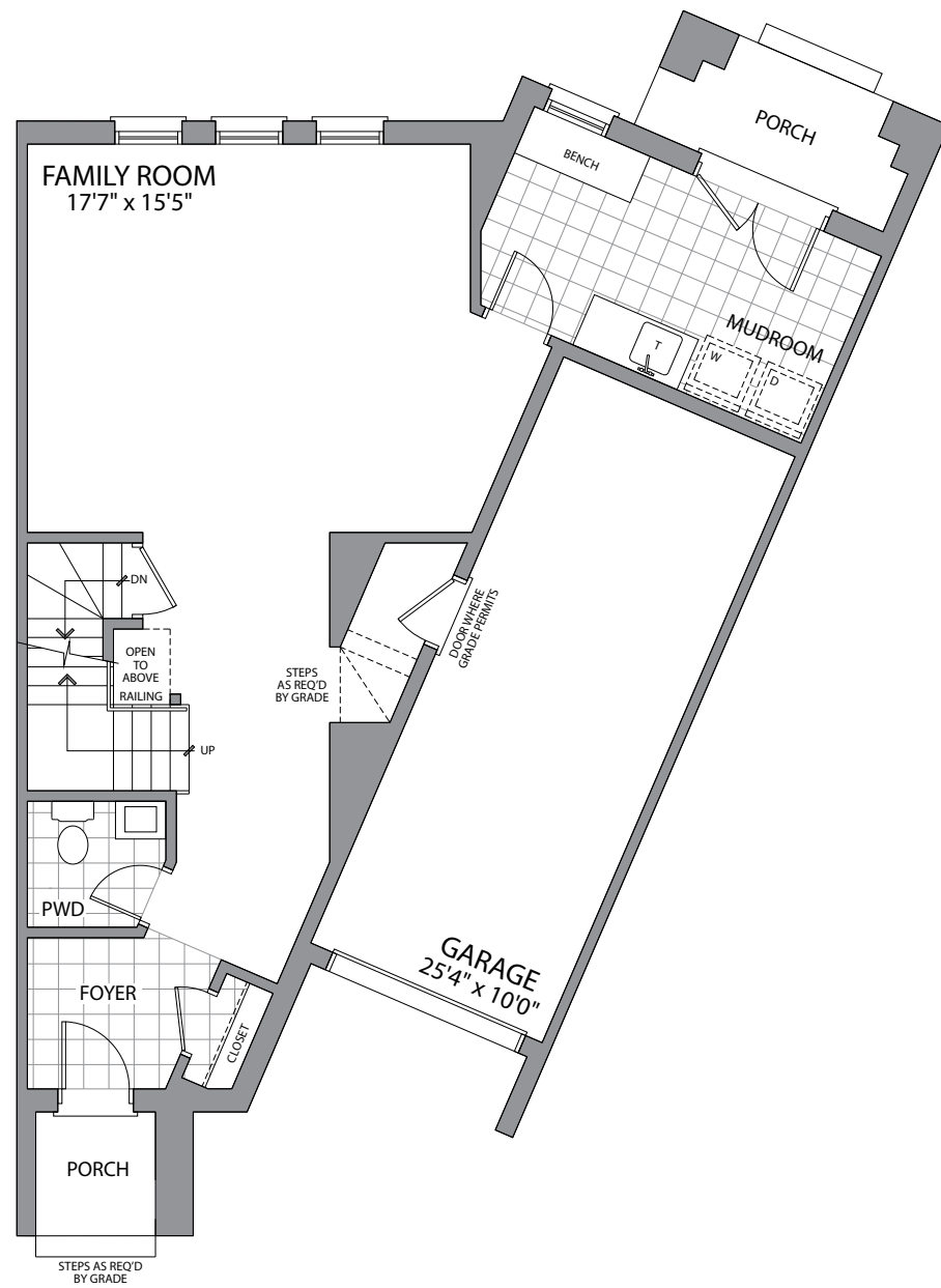
FIRST FLOOR ELEVATION A & B
