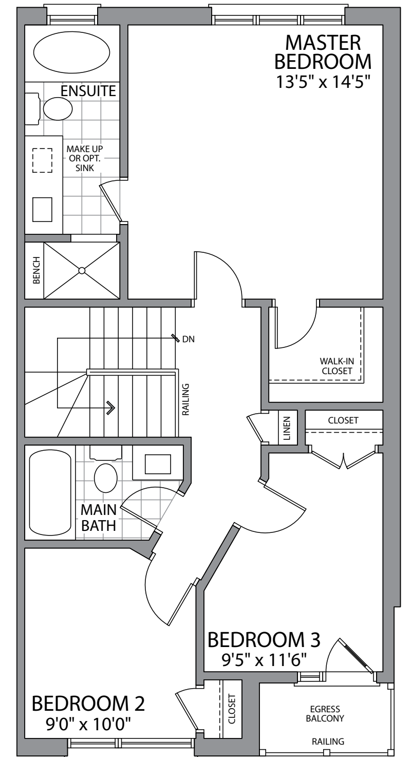
THIRD FLOOR ELEVATION A & B
