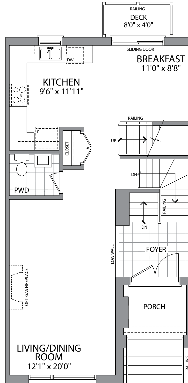
SECOND FLOOR ELEVATION A & B
