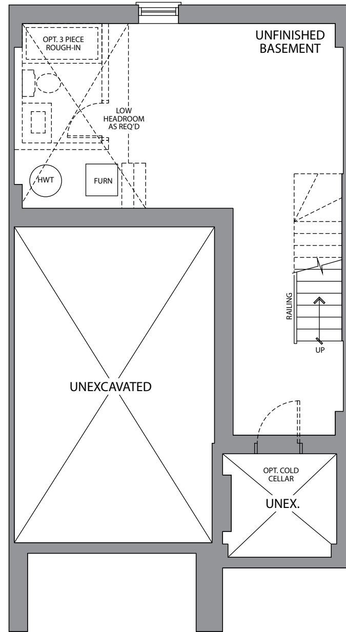
BASEMENT ELEVATION A & B
