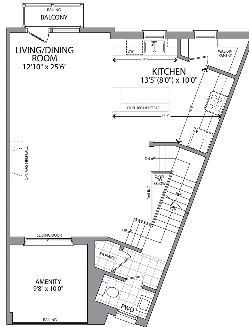
SECOND FLOOR ELEVATION A & B
